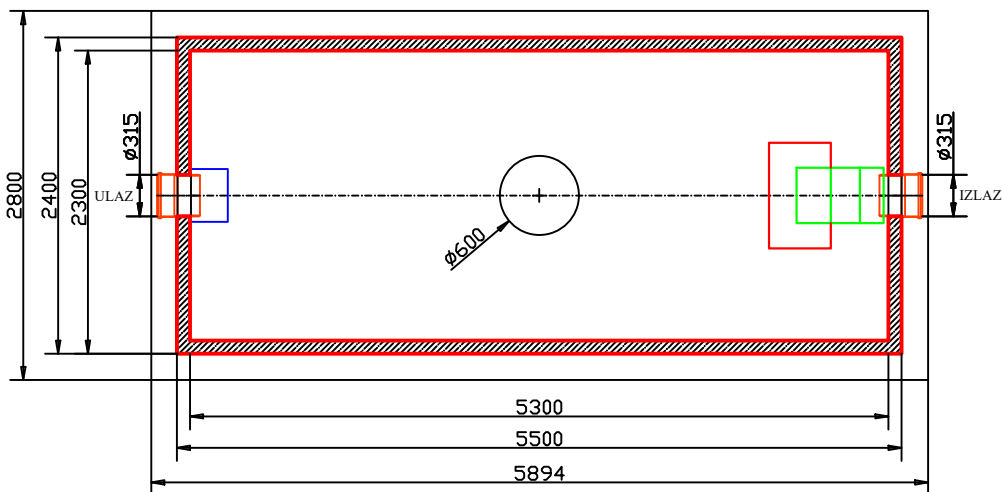
BASE PLATE DIMENSIONS
