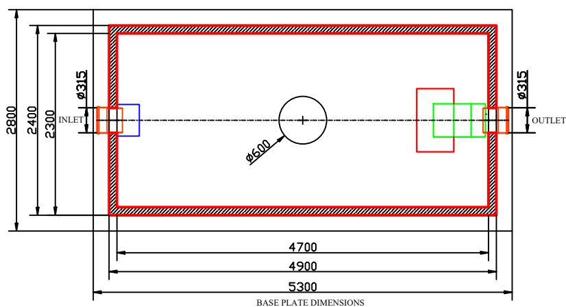
BASE PLATE DIMENSIONS
