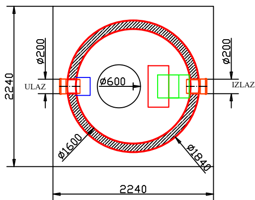
BASE PLATE DIMENSIONS
